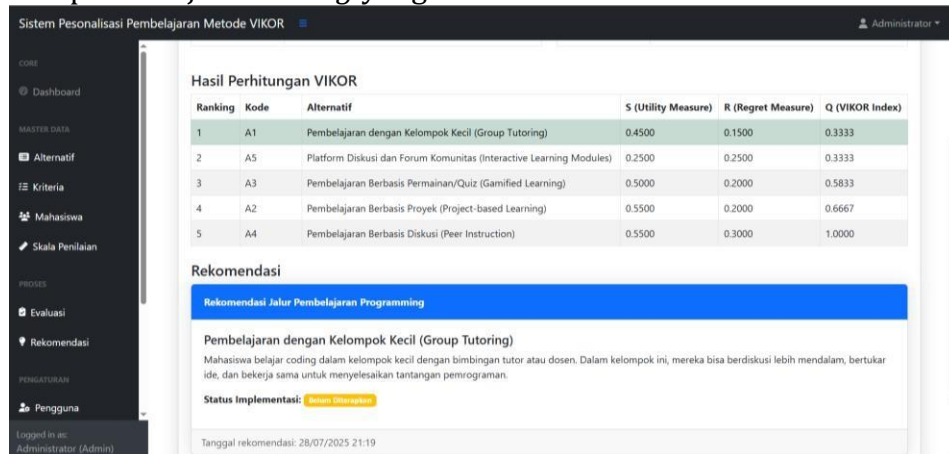
Gambar 7. Halaman Detail Hasil Rekomendasi
